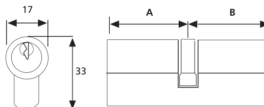
Economy Euro Profile Cylinder
