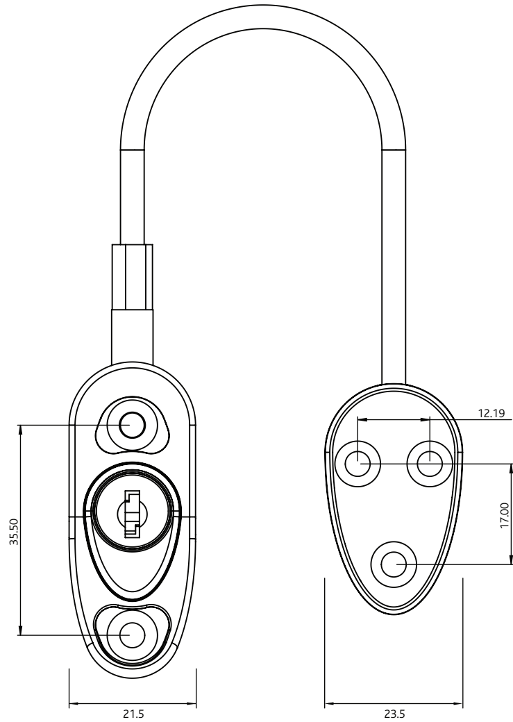
Diagram not to scale. All dimensions are in mm and are nominal. ERA reserves the right to change specification without notice It is the responsibility of the window and door manufacturer to ensure that the finished product meets any required safety and performance specification.
