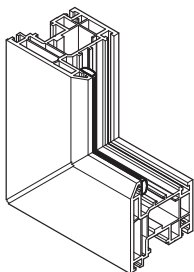
Traditional Welded Joint
